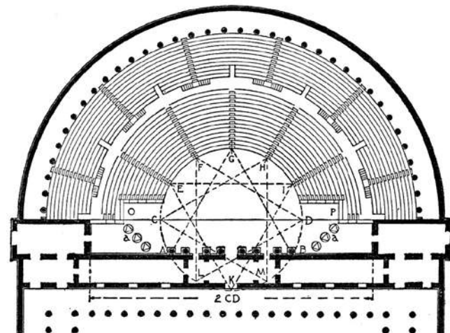
Gubbio Roman Theater - Geometric analysis
